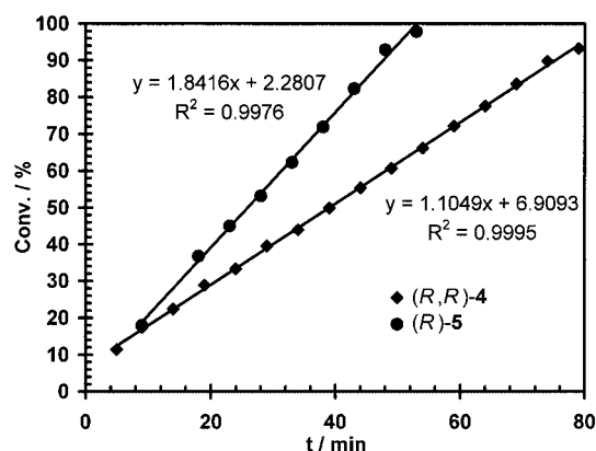
Figure 4. Hydroamination/cyclization of 8 (0.63 M) with 1 mol % ( R,R )- 4 (= 2 mol % La) and 2 mol % ( R )- 5 at 25 °C in C_6D_6 .
