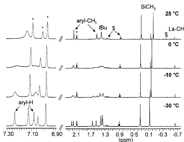
Figure 1. Variable temperature ^1\text{H} NMR spectra of (R,R)\text{-4} in [\text{D}_8]\text{toluene} (*) showing the aliphatic (right) and aromatic region (left, threefold expanded) [ \text{S} = n\text{-pentane} , \text{§} = \text{CH}_2(\text{SiCH}_3)_2 ]
