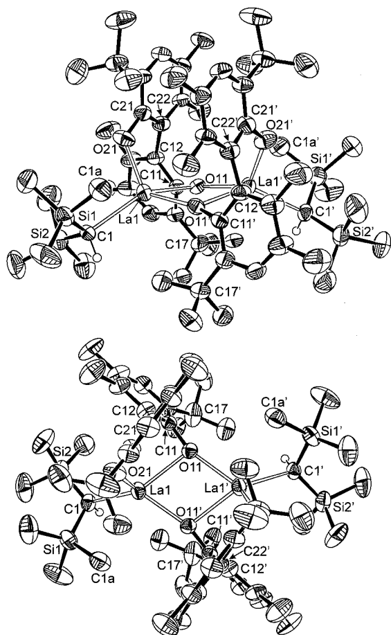
Figure 2. ORTEP diagram of the molecular structure of ( R,R )- 4 (top) and alternative view from the top (bottom); thermal ellipsoids are drawn at the 50% probability level; hydrogen atoms, except for those on C1 and C1', as well as one position of the disordered tert -butyl group on C17 have been omitted for the sake of clarity
