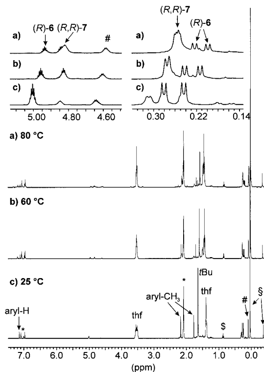
Figure 3. ^1\text{H} NMR spectrum of the equilibrium between (R) -6 and (R,R) -7 in [\text{D}_8]\text{toluene} at: a) 80^\circ\text{C} , b) 60^\circ\text{C} and c) 25^\circ\text{C} [ \# = \text{HN}(\text{SiHMe}_2)_2 , \$ = \text{CH}_2(\text{SiMe}_3)_2 , \$ = \text{pentane} ]
